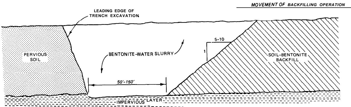
Figure 5-4. Installation of a slurry cutoff trench.
